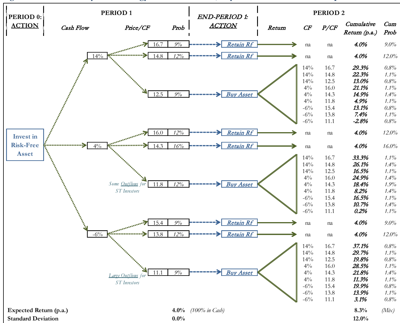
Figure 7: Schematic of Dynamic Strategy B – Invest in Cash; Buy Asset End-Period 1 If Multiple Low
